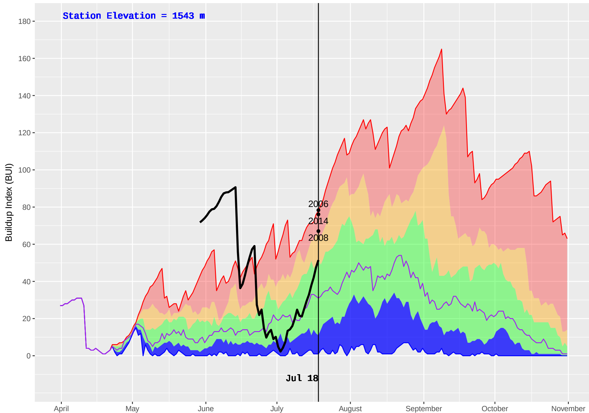
CAHILTY (253) : Historical (1987–2016) and Current (2018) Daily Buildup Index (BUI)
